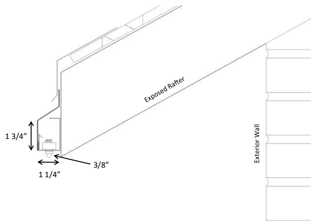
Rafter Board Installation
