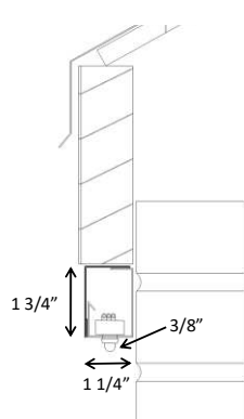
For Fascia Board Installation
